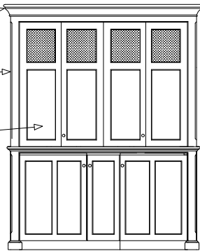
UNIT CODE: UK68B-CSR-MH (SHOWN WITH ALL LOWER DOOR OPTION)
